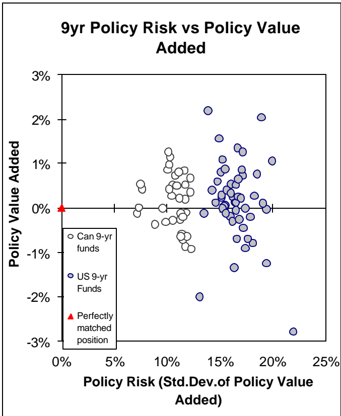
Figure 4: Policy Value Added vs Policy Risk
